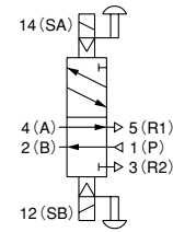
HEA10F6 [De-energized condition after energizing solenoid 12 (SB)]
